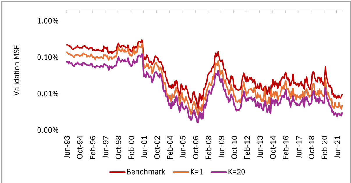
Figure D1: Mean squared error of bid-ask spread approximation
