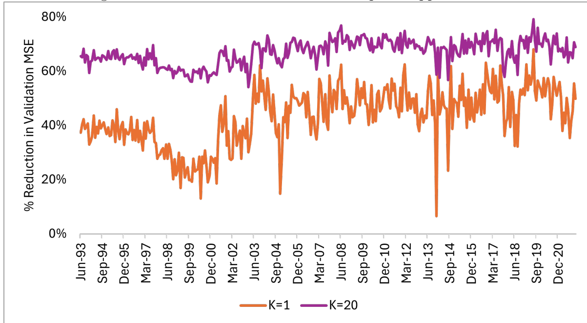
Figure D2: Reduction in MSE of bid-ask spread approximation
