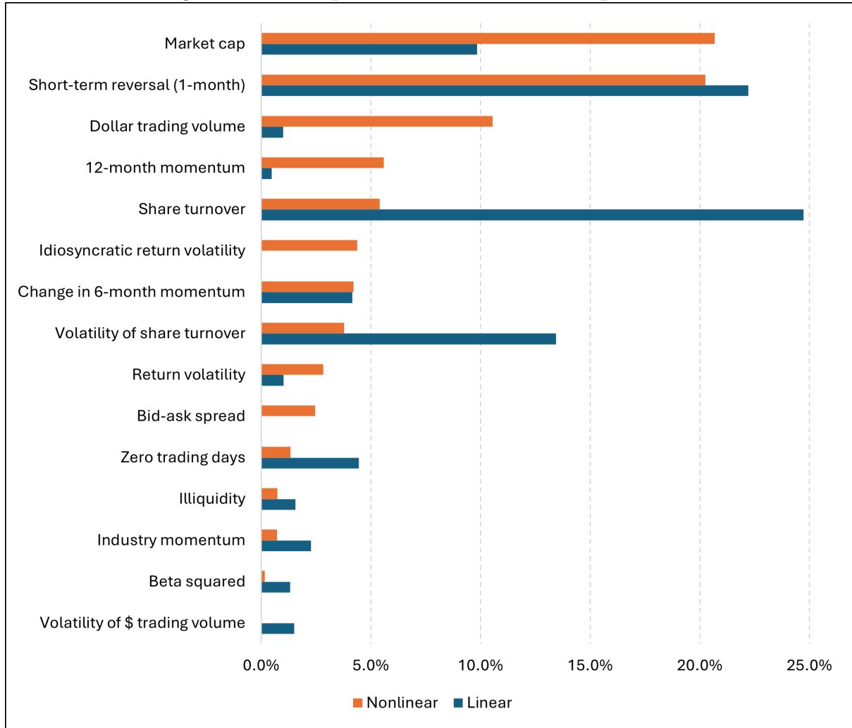
Figure 4: In-sample statistical feature importance
