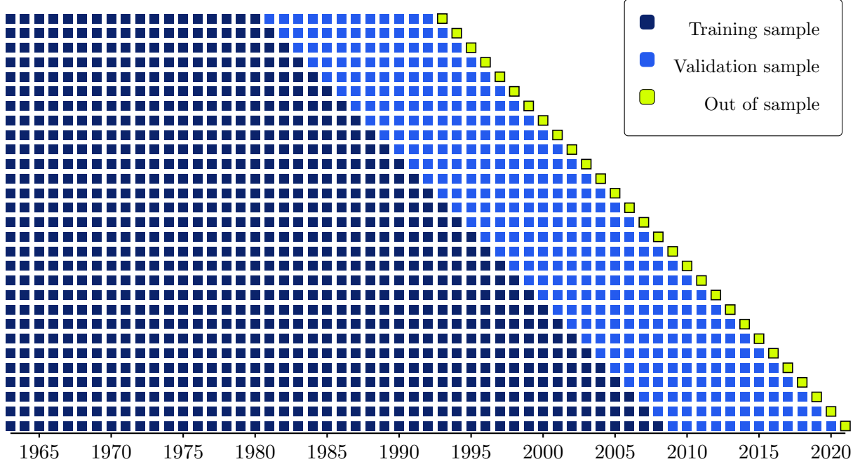
Figure 1: Training and validation of return prediction model
