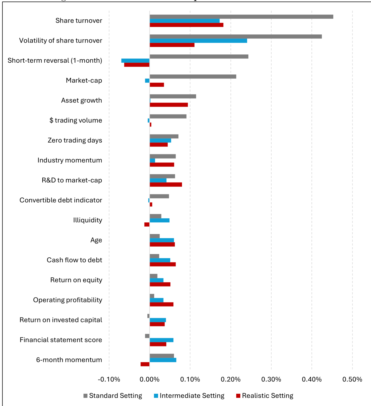
Figure 6: Economic feature importance in a linear model
