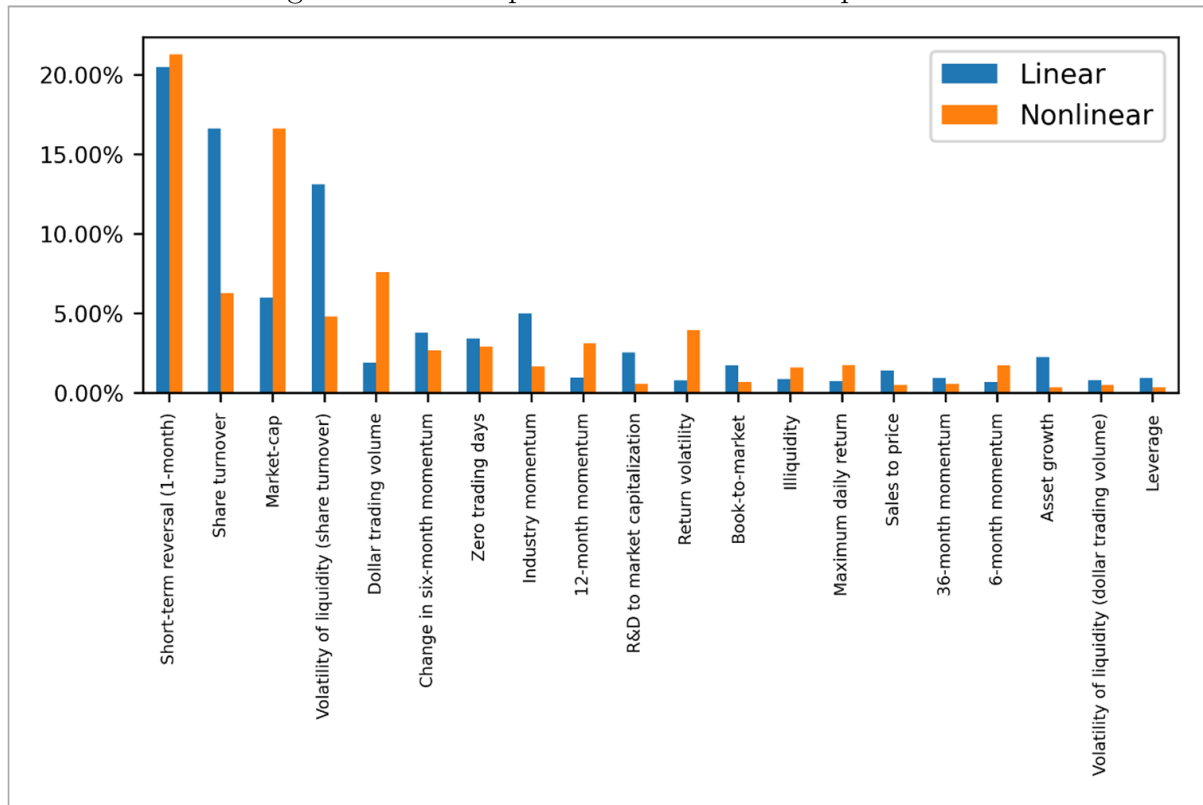
Figure F1: In-sample statistical feature importance
