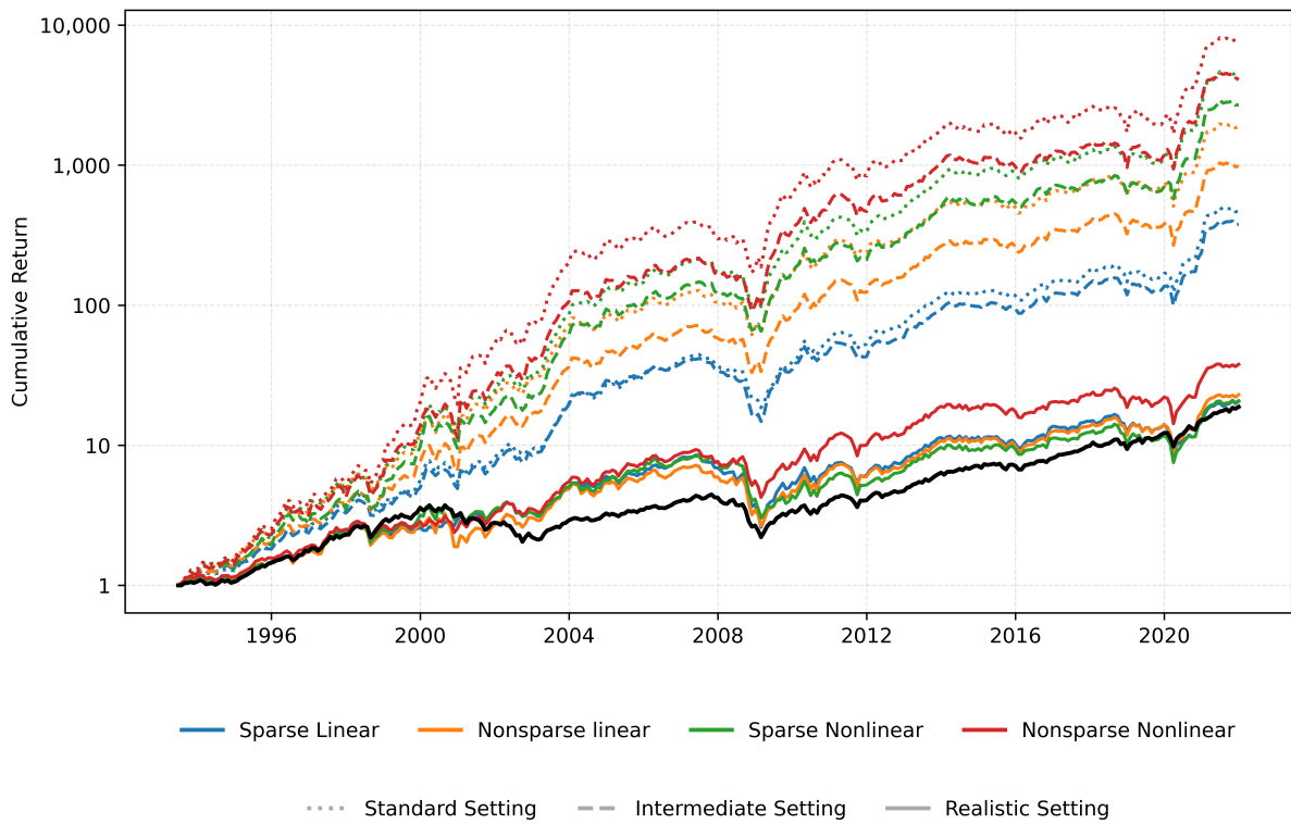
Figure C2: Cumulative returns of L/O strategies across different settings
